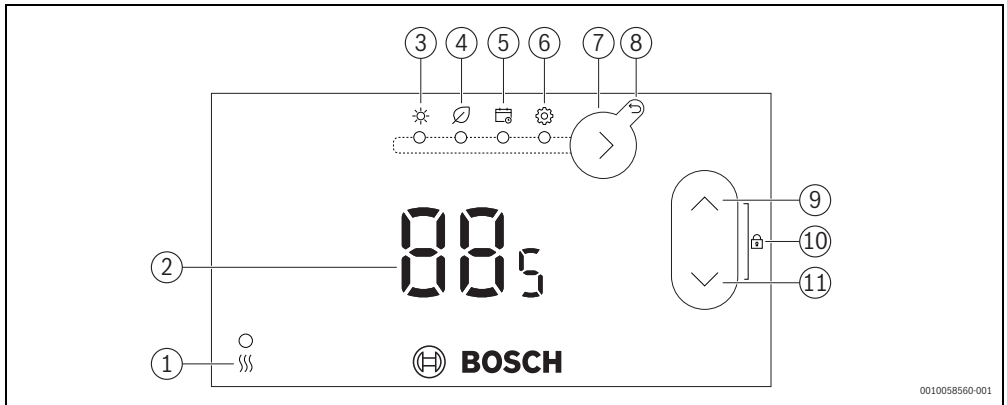
Fig. 1 Control elements
