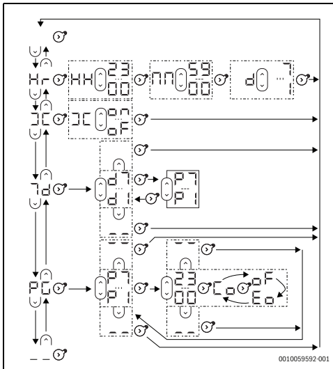
Fig. 3 Appliance settings menu flowchart
