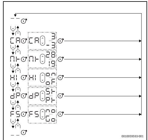
Fig. 4 Expert menu flowchart
